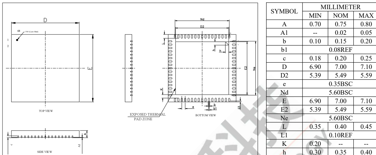
Figure 4-1 AC7925A Package
